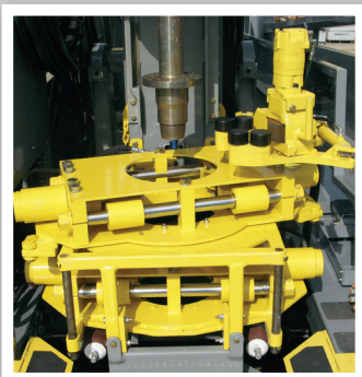
Break out wrench system with rod spinner
